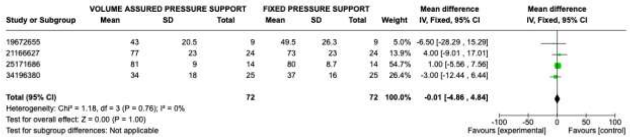
Figure 8. Forest plot of mean difference with confidence interval for post-treatment VAS Comfort Scale
