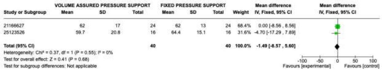
Figure 7. Forest plot of mean difference with confidence interval for post-treatment St. George Respiratory Questionnaire
